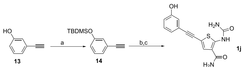
Scheme 2. Reagents and conditions: (a) TBDMSCl, imidazole, DMF, rt, 86%; (b) 2 , PdCl 2 [( i -Pr 2 PC 3 H 4 ) 2 Fe], CuI, i -Pr 2 NEt, EtOH/DMA, 75 °C, 70%; (c) TBAF, THF, rt, 42%.
