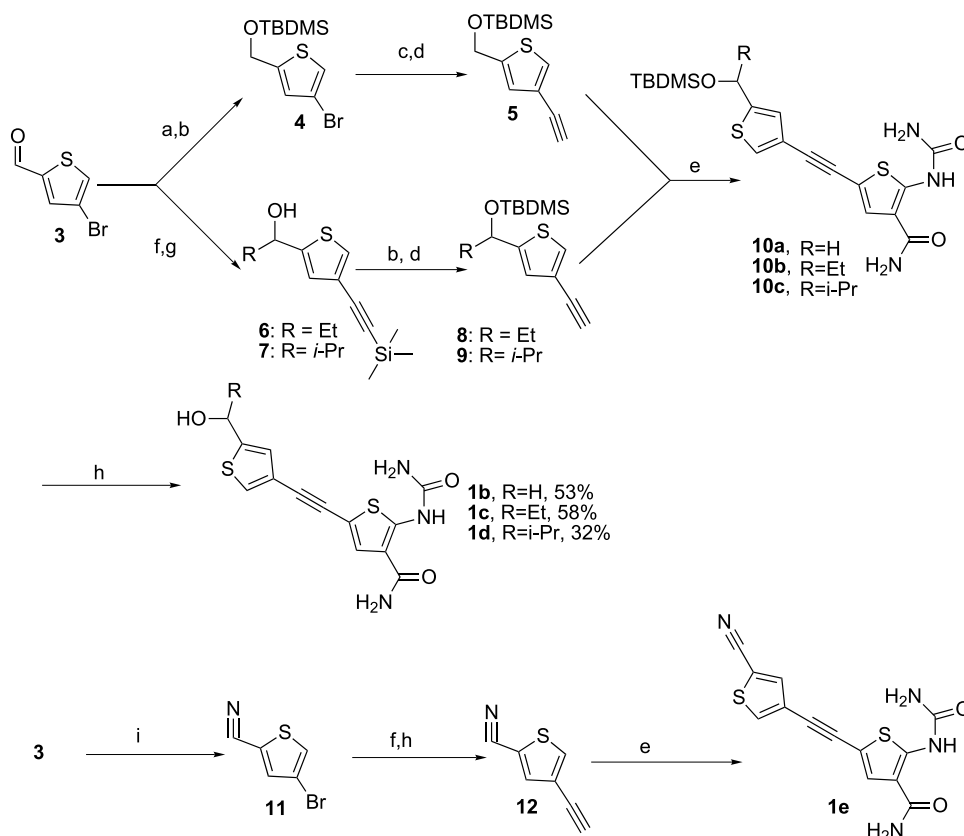
Scheme 1. Reagents and conditions: (a) NaBH 4 ; (b) TBDMSCl, imidazole, DMF; (c) TMSCH, Pd(PPh 3 ) 4 , CuI, Et 3 N, THF, 70%; (d) NaOH (1 M, H 2 O), MeOH, rt, 2 h; (e) 2 , PdCl 2 [( i -Pr 2 PC 5 H 4 ) 2 Fe], CuI, i -Pr 2 NEt, EtOH/DMA, 65–75 °C, 37–76%; (f) TMSCH, PdCl 2 (PhCN) 2 , PPh 3 , CuI, i -Pr 2 NH, benzene, 97%; (g) RMgBr, THF; (h) TBAF, THF, rt, 32–58%; (i) (1) NH 2 OH·HCl, Et 3 N, (2) phthalic anhydride, 99%.
