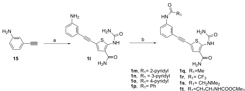
Scheme 3. Reagents and conditions: (a) 2 , PdCl 2 (PhCN) 2 , ( i -Pr 2 ) 2 Fc, CuI, i -Pr 2 NEt, EtOH/DMA, 75 °C, 17%; (b) RCO 2 H, Me 2 EtN, HBTU, DMF, rt, 62–93%.
